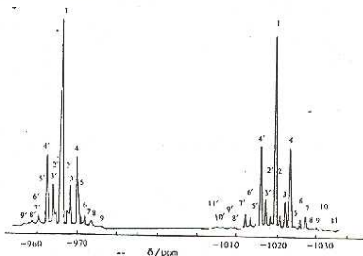
图4 \text{Pb}_3\text{Sn}_6^{4-} (左) 及 \text{Pb}_4\text{Sn}_5^{4-} (右) 的 ^{119}\text{Sn} NMR 谱 Fig.4 ^{119}\text{Sn} spectra of \text{Pb}_3\text{Sn}_6^{4-} (left) and \text{Pb}_4\text{Sn}_5^{4-} (right)
